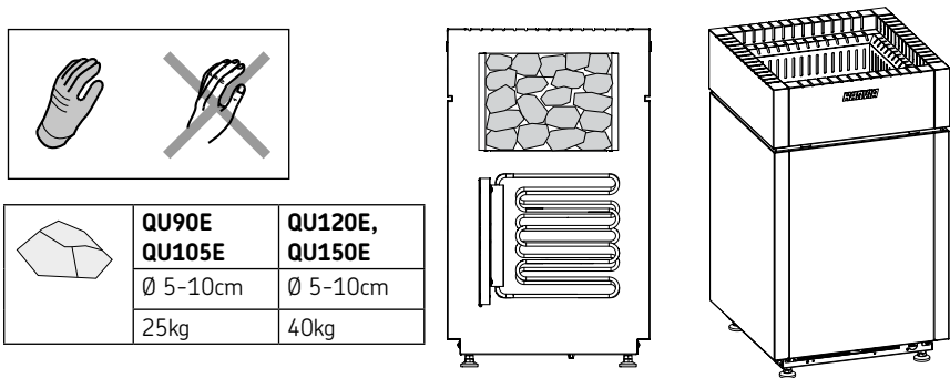
Figure 9. Placing of sauna stones
